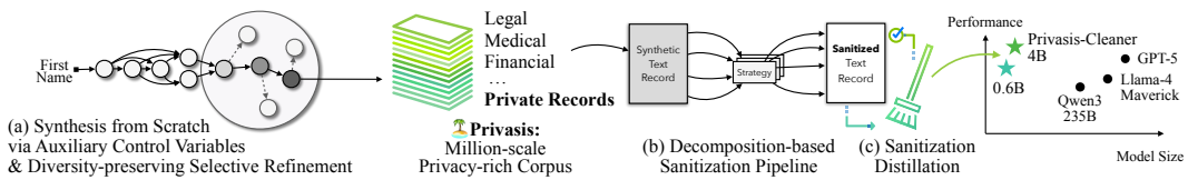
Figure 1: PRIVASIS, the Privacy Oasis Dataset: We synthesize the first publicly-available million-scale dataset with diverse private information, entirely from scratch. (a) Using auxiliary control variables, we initialize a text record draft containing rich private information and then selectively refine it while preserving the overall diversity of the record set (§2). (b) Based on this, we construct a parallel corpus for text sanitization using a decomposition-based sanitization pipeline (§3). (c) On this parallel corpus, we train compact sanitization models ( \leq 4\text{B} ) that outperform GPT-5 (§4).
